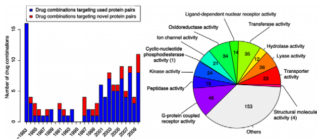
Figure 2. Historical distribution of drug combinations with respect to novel target combinations. (a) Distribution of pairwise drug combinations that target novel protein pairs or ones that are also targeted by previous combinations for the time between 1984 and 2010. (b) Distribution of drug targets with respect to molecular functions from Gene Ontology. doi:10.1371/journal.pcbi.1002323.g002
